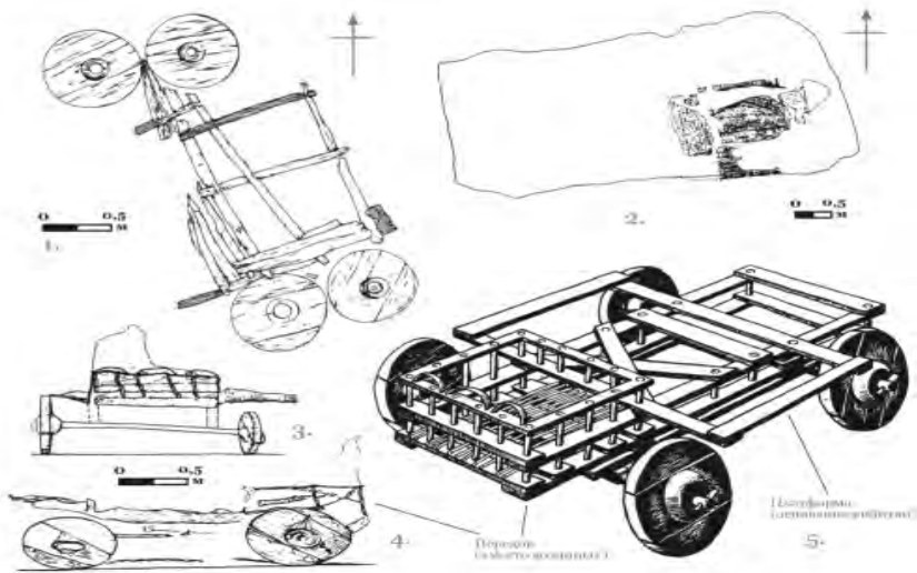
Fig. 3. Reconstruction of Novotitorovo four-wheels covered wagon (van) in Northern Caucasias (Gay 2000).
